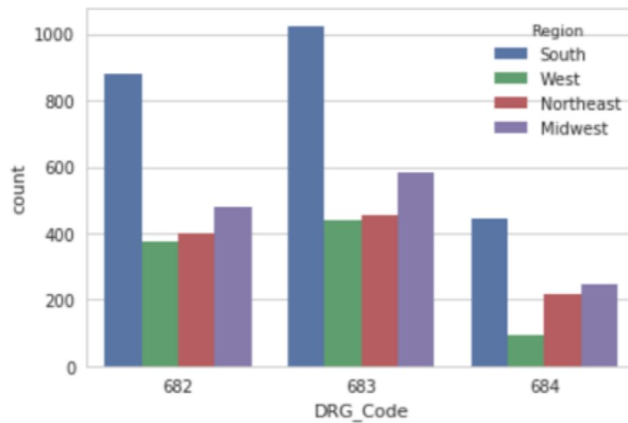
countplot
