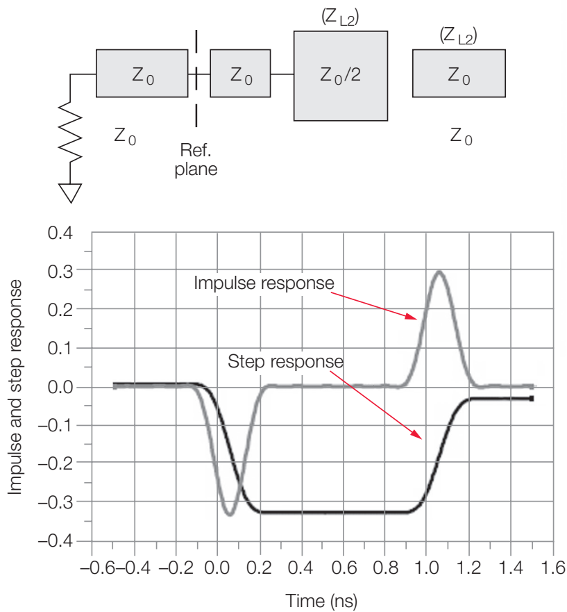
Figure 8. Showing a low-pass step and impulse responses of impedance changes (circuit shown above)
